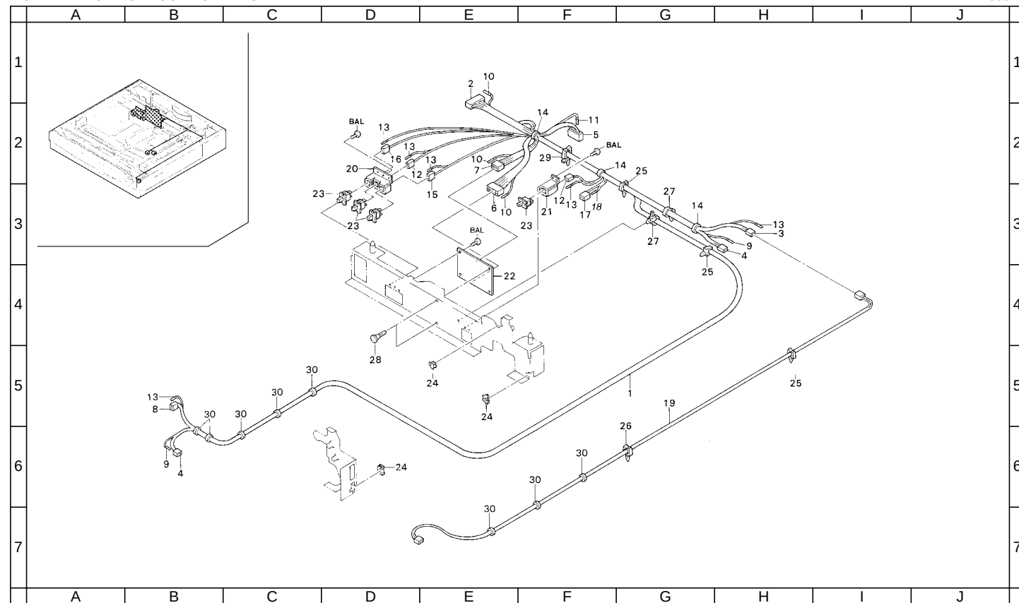
FIG. 4 ELECTRICAL COMPONENTS
