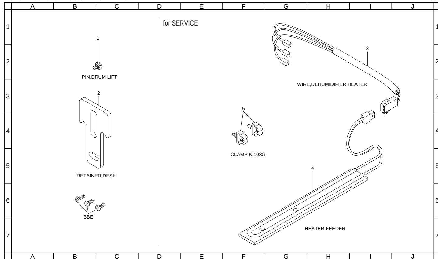
FIG. 5 ACCESSORIES & SERVICE PARTS
